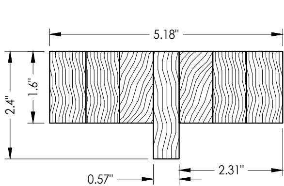
20 FRAME HEADER
