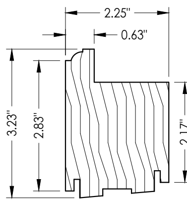
26 BOTTOM SASH BOTTOM RAIL
