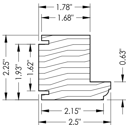
25 SASH STILE
